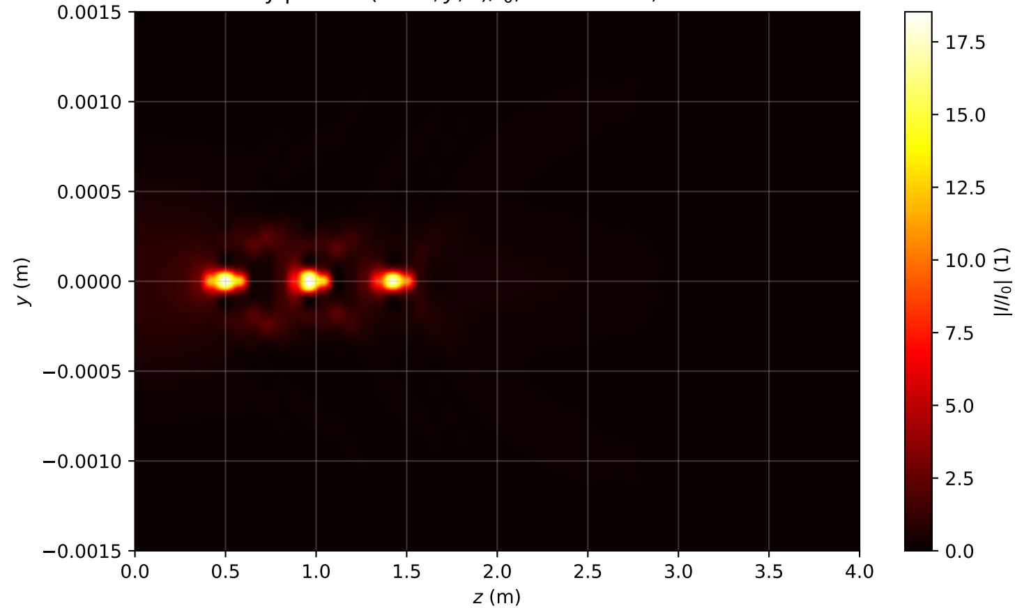
Intensity profile I(x=0, y, z)/I_0 , P_{in}=6.0P_{cr} , artificial time
